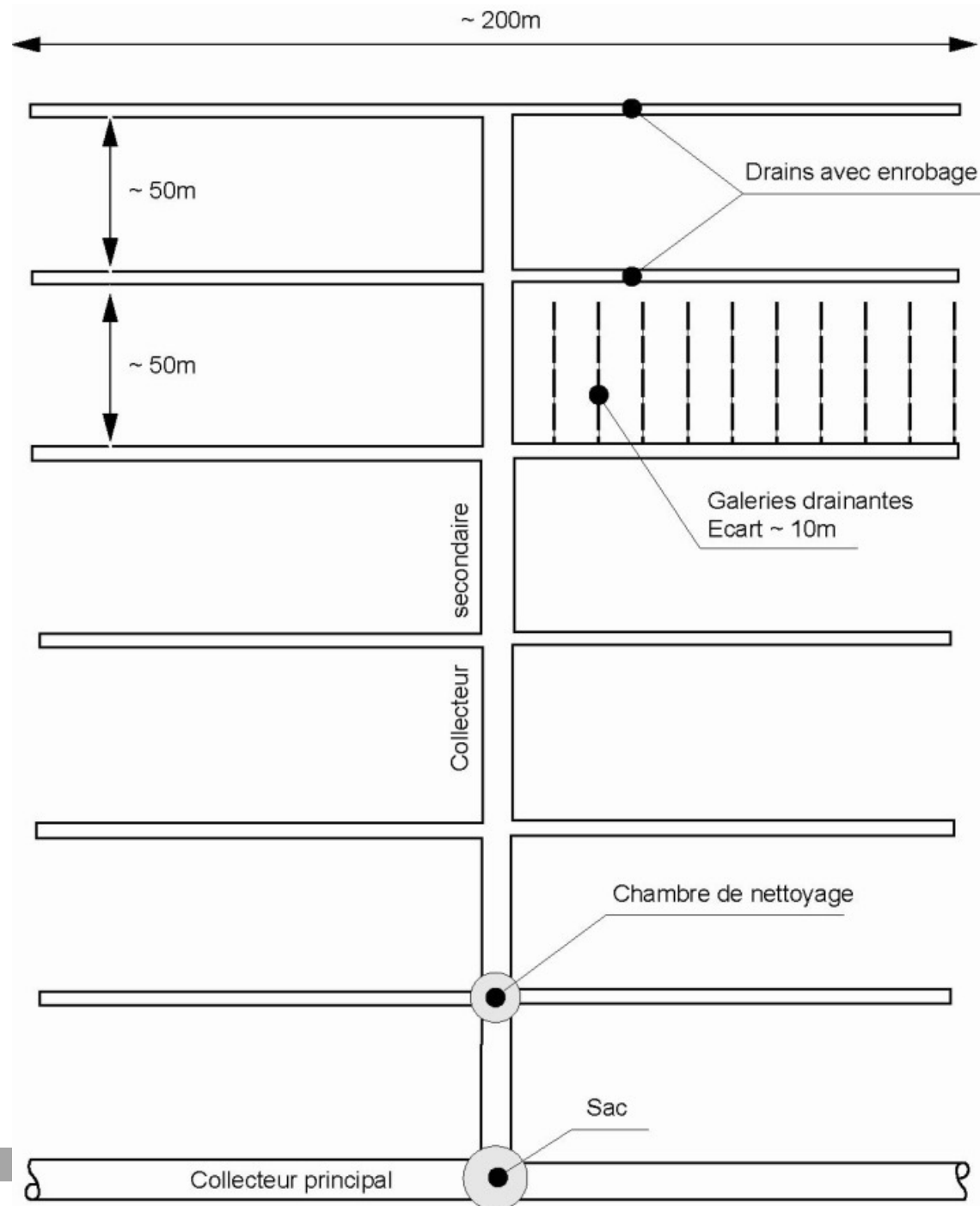
Schematic diagram of drainage using drainage galleries
